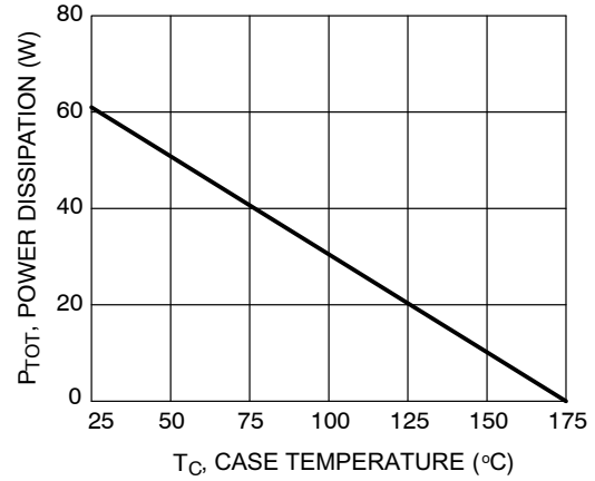
Figure 4. Power Derating
