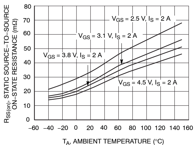
Figure 11. R_{SS(on)} - T_A
