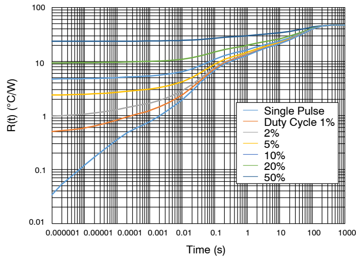
Figure 13. Thermal Response
