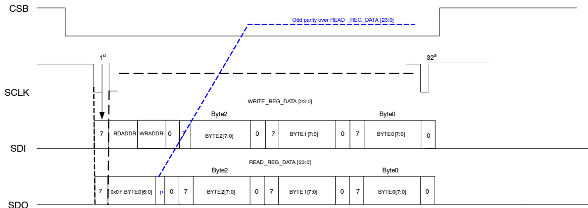
Figure 17. SPI Frame Format
