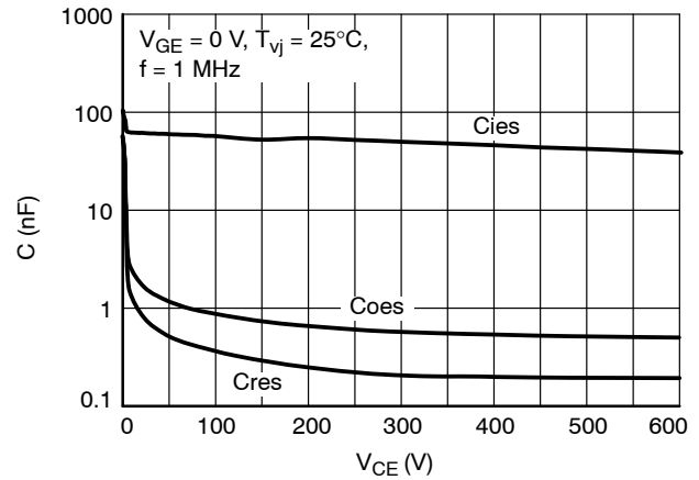
Figure 6. Capacitance Characteristic
