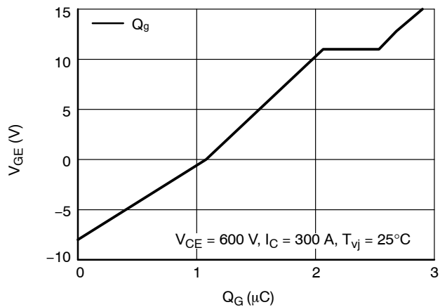
Figure 5. Gate Charge Characteristic
