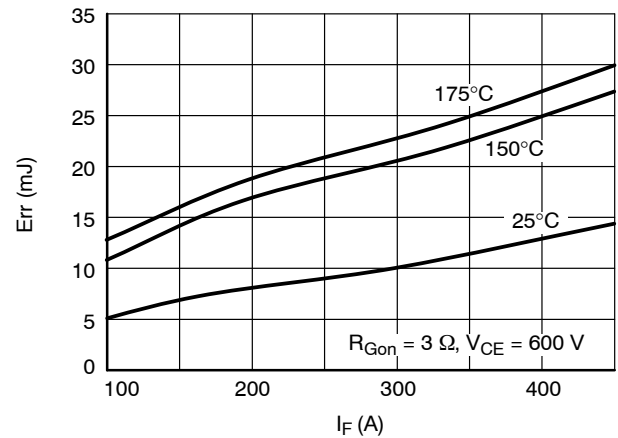
Figure 16. Diode Switching Losses vs. I_F
