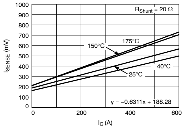
Figure 21. Current Sensor Characteristics
