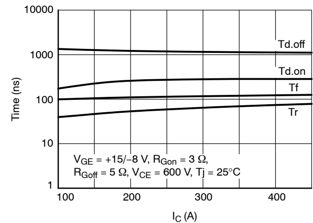
Figure 12. IGBT Switching Times vs. I_C , T_{vi} = 175^\circ\text{C}
