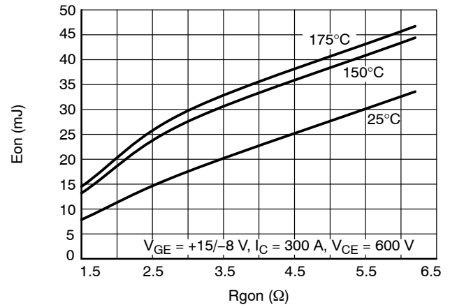
Figure 8. IGBT Turn-on Losses vs. R_{Gon}
