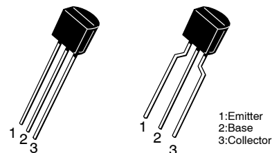
TO-92 3 CASE 135AN
