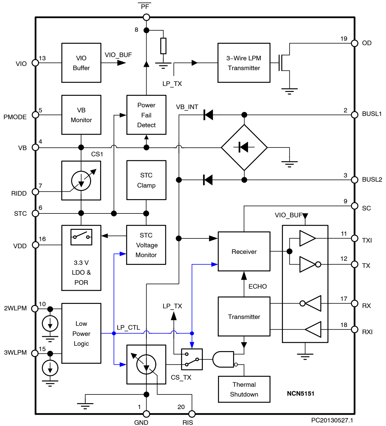
Figure 2. NCN5151 Block Diagram
