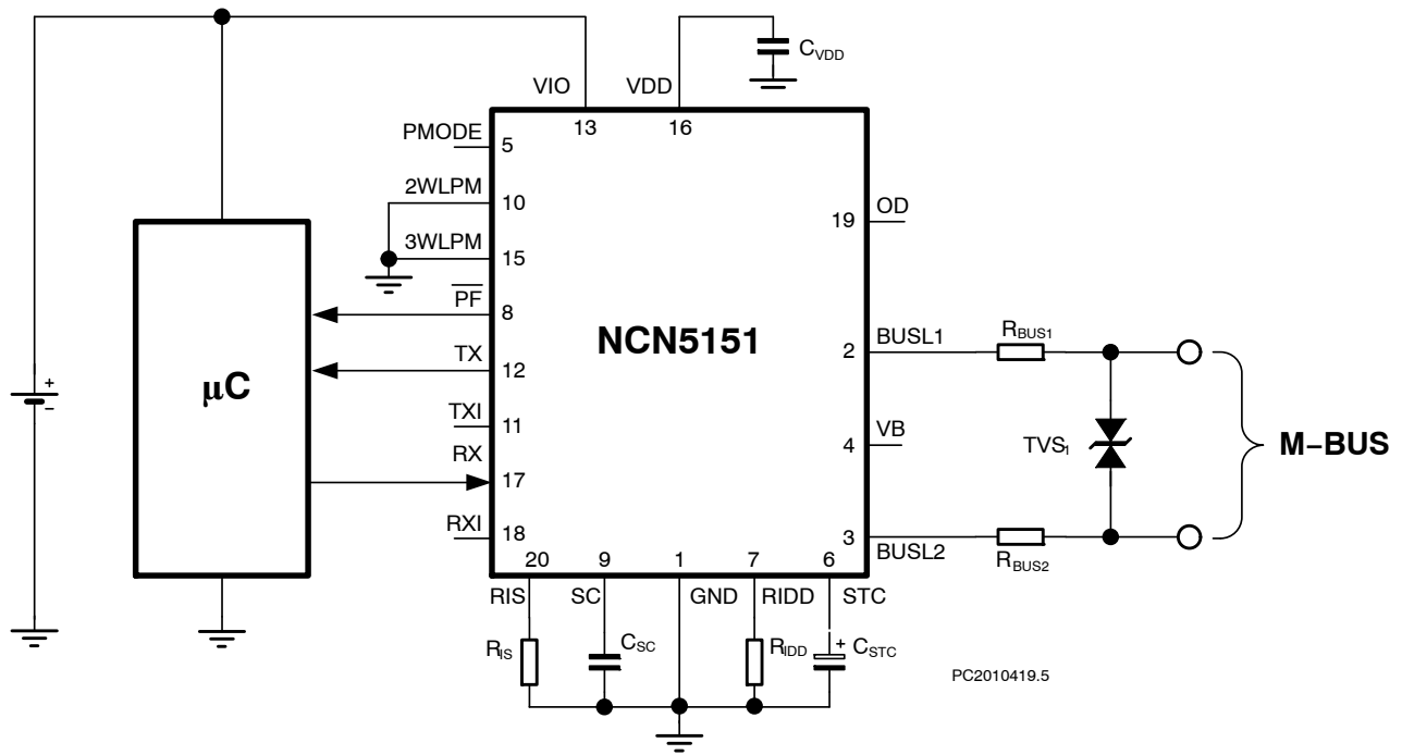
Figure 4. Application Schematic with External Power Supply
