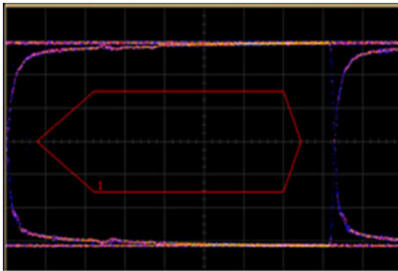
Figure 13. USB 1.1 Full Speed Eye Diagram
