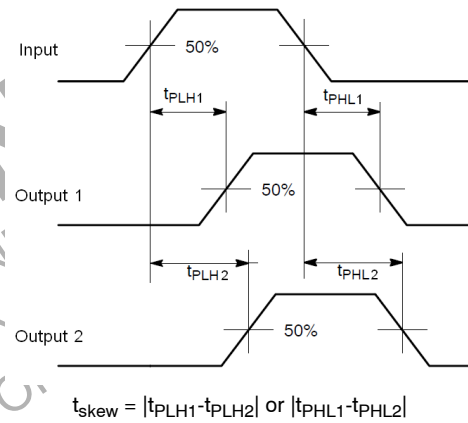
Figure 6. Bit-to-Bit and Channel-to-Channel Skew
