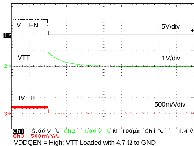
Figure 22. VTT Shutdown Waveforms
