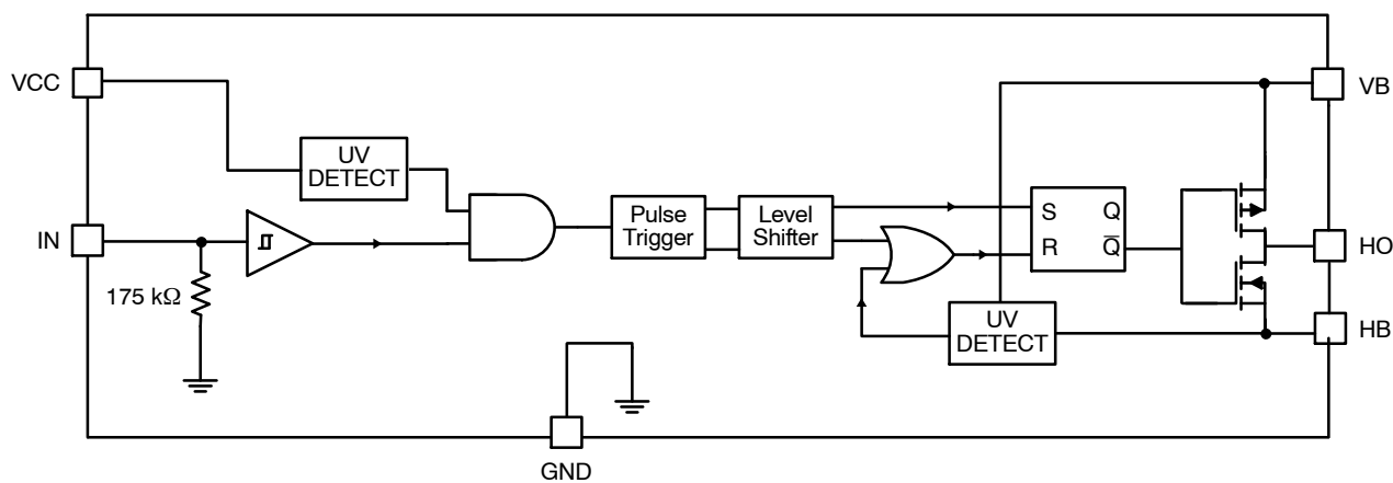
Figure 3. Internal Block Diagram for NCV51313
