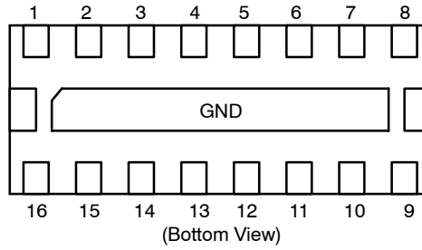
Figure 3. Pin Diagram
