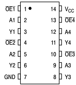
(Top View) Figure 2. Pinout: 14-Lead Packages
