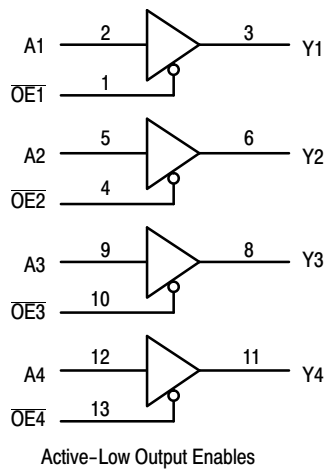
Active-Low Output Enables Figure 1. Logic Diagram
