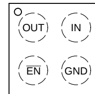
WLCSP (Top Views)
