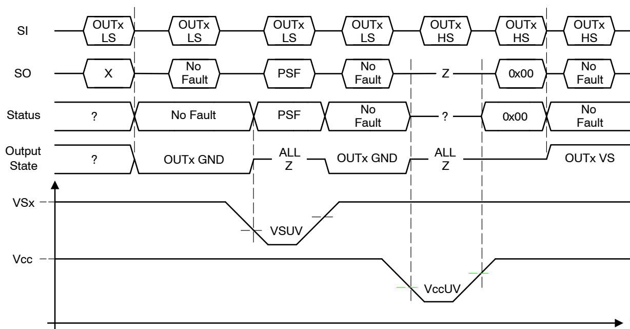
Figure 19. Undervoltage Timing
