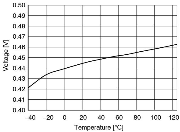
Figure 8. V_{Chyst} vs. Temperature
