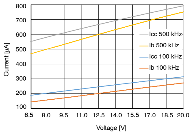
Figure 35. Current Consumption vs. Voltage. Cload = 0 nF
