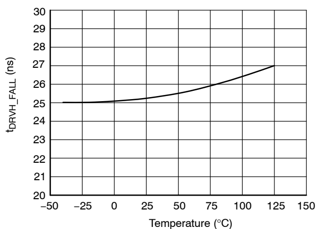
Figure 28. High Side Driver Fall Time t_{DRVH\_FALL} from 90% to 10% of DRVH Signal
