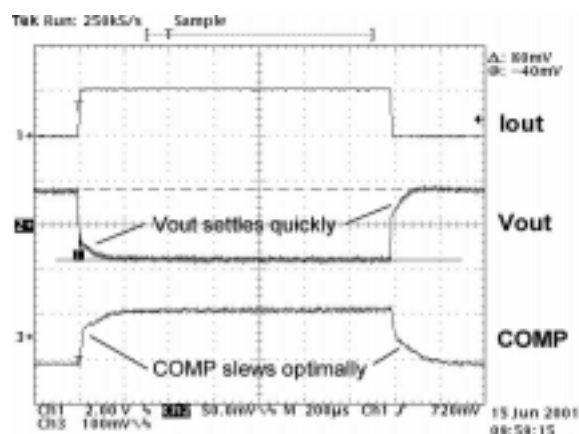
Figure 39. COMP Tuning, Bandwidth Too High
