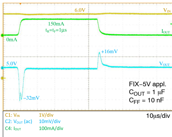
Figure 39. Load Transient Response (FIX-5V, V_{IN} = 6.0\text{ V} , C_{OUT} = 1\text{ }\mu\text{F} )
