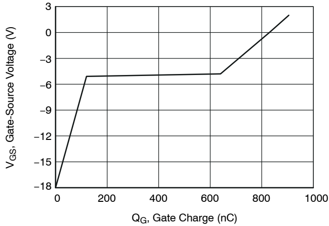
Figure 15. Typical Gate Charge at V_{DS} = 800\text{ V} and I_D = 100\text{ A}
