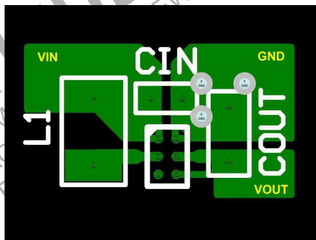
Figure 20. WLCSP Suggested Layout (Top View)
