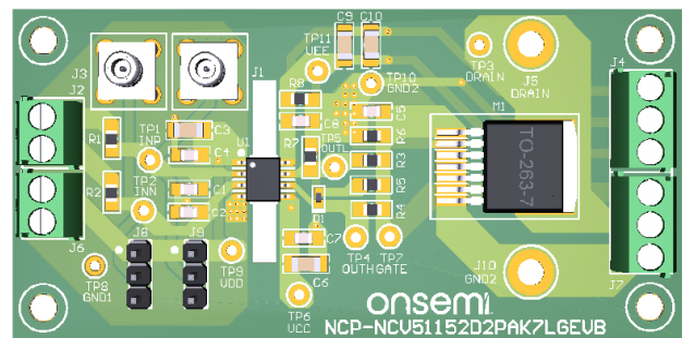
Figure 52. 3-D PCB View
