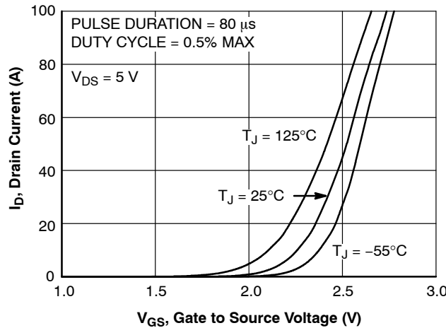
Figure 18. Transfer Characteristics
