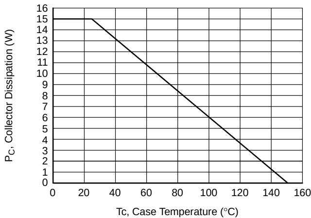
Figure 12. P_C - T_c
