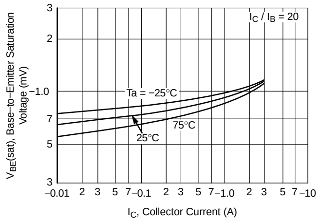
Figure 9. V_{BE(sat)} - I_C
