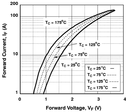
Figure 21. Forward Characteristics
