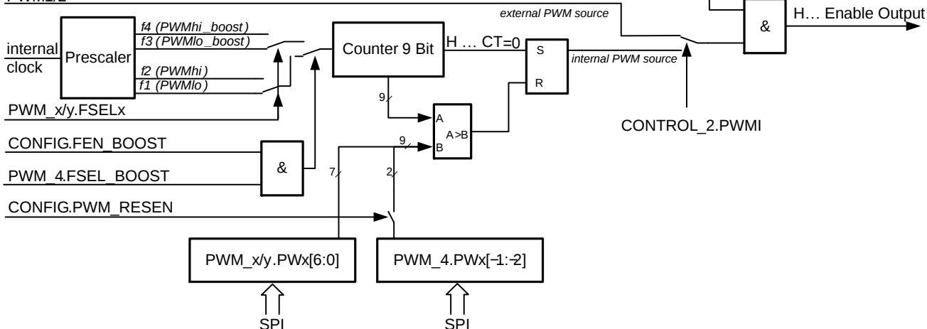
Figure 5. PWM Generation Diagram
