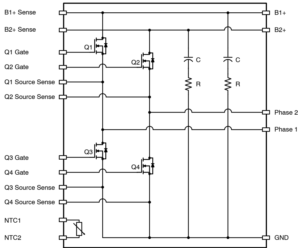
Figure 2. Schematic
