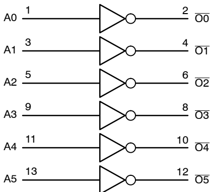
Figure 1. Logic Diagram
