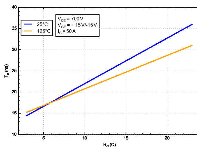
Figure 23. Typical Reverse Recovery Time vs. RG
