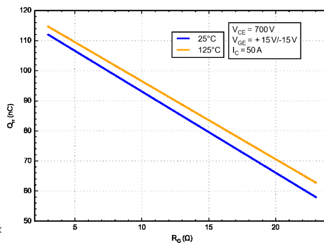
Figure 25. Typical Reverse Recovery Charge vs. RG
