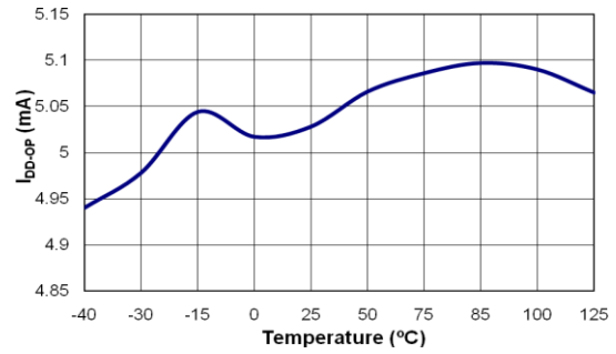
Figure 8. Operating Current
