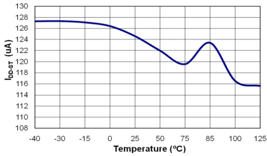
Figure 7. Startup Current
