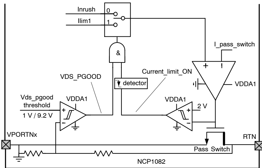
Figure 13. Inrush and Ilim1 Selection Mechanism
