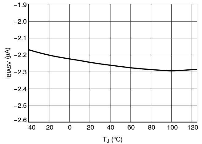
Figure 13. IBIASV at VCC = 15 V, VSENS > VSENSBIASHTH
