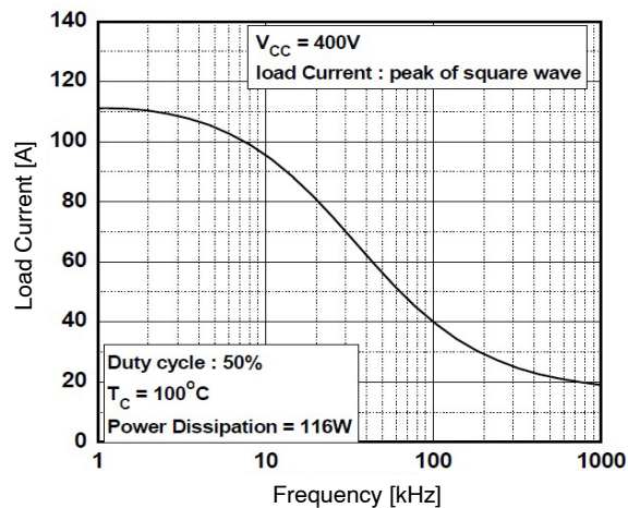
Figure 18. Load Current vs. Frequency
