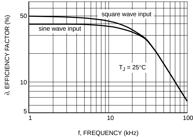
Figure 10. Rectification Waveform Efficiency
