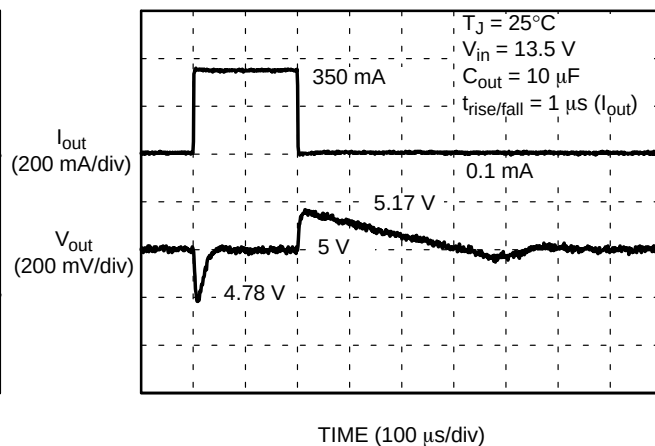
Figure 30. Load Transients
