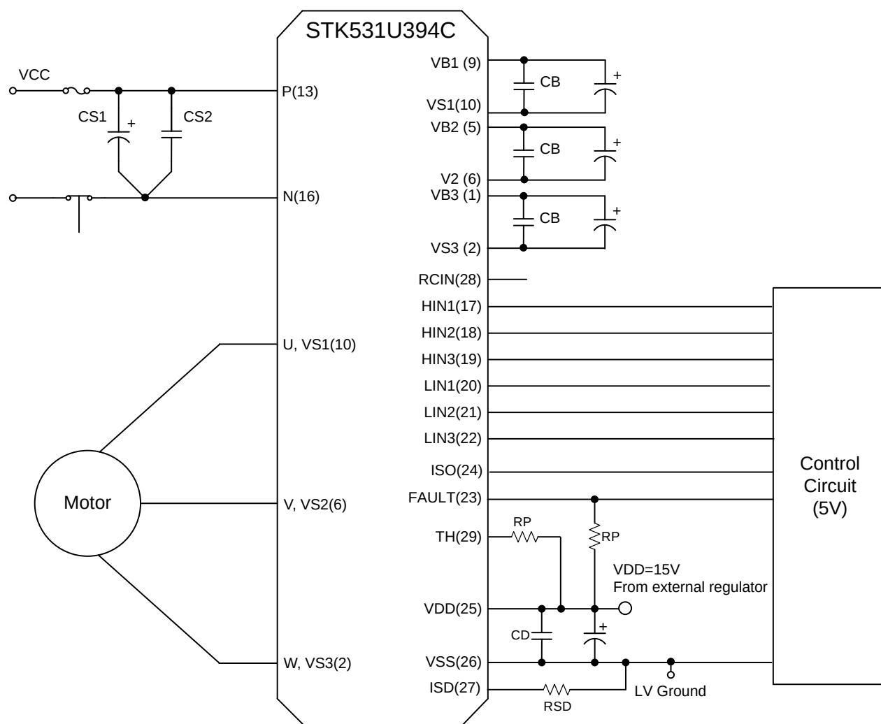
Figure 2. Application Schematic
