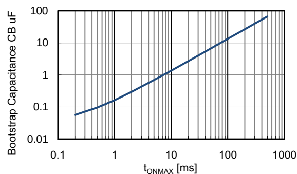
Figure 7. Bootstrap Capacitance versus t_{ONMAX}
