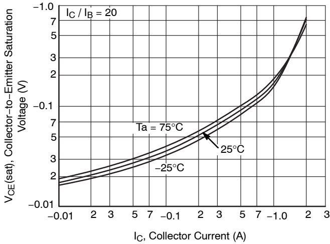
Figure 14. V_{CE(sat)} - I_C (PNP)
