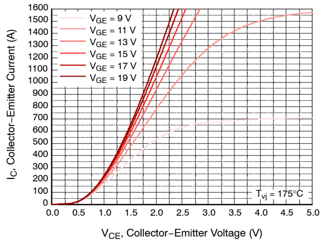
Figure 2. Output Characteristic, IGBT (Typ.)
