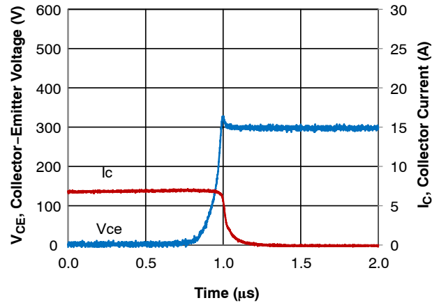
Figure 11. Turn-off Waveform T j = 100°C, V CC = 300 V
