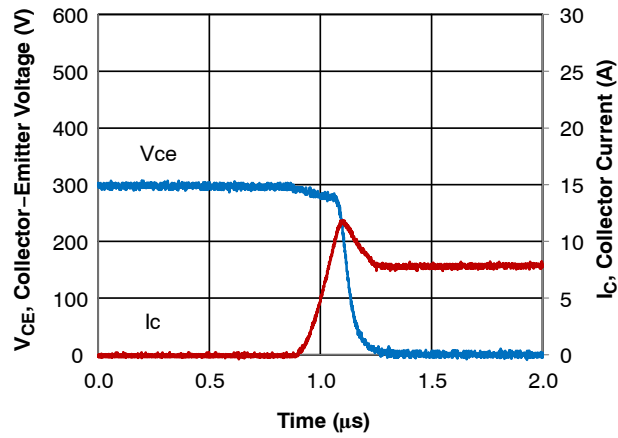
Figure 10. Turn-on Waveform T j = 100°C, V CC = 300 V
