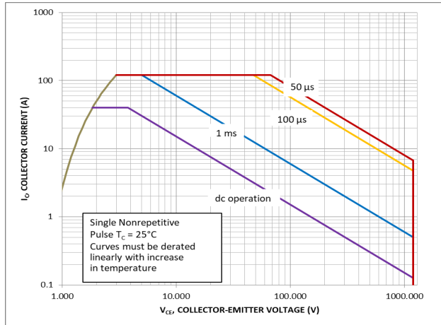
Figure 8. FBSOA
