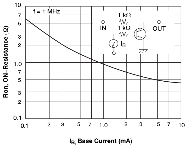
Figure 10. R_{on} - I_B
