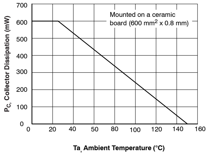
Figure 11. P_C - T_a
