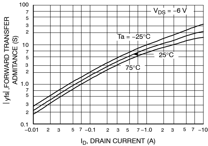
Figure 6. |y_{fs}| - I_D
