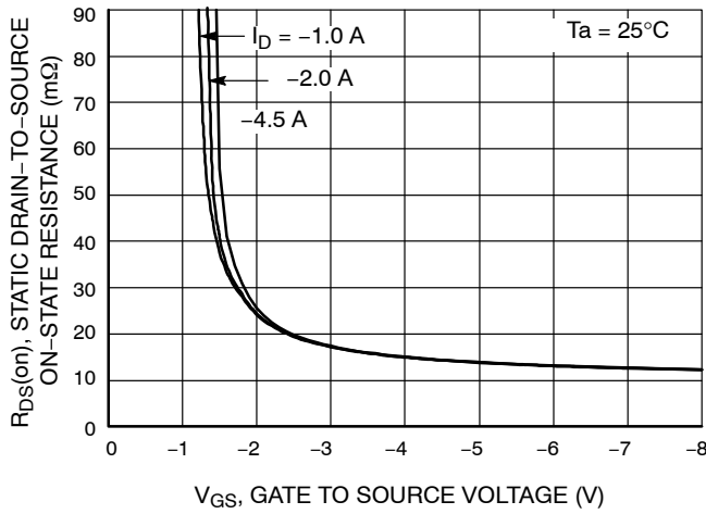
Figure 4. R_{DS(on)} - V_{GS}
