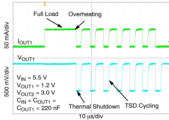
Figure 53. Short-Circuit and Thermal Shutdown
