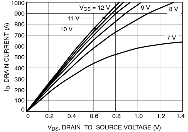
Figure 4. Saturation Characteristics
