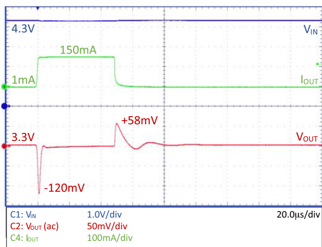
Figure 17. Load Transient – NCV8730–3.3 V, C_{OUT} = 1\text{ }\mu\text{F}
