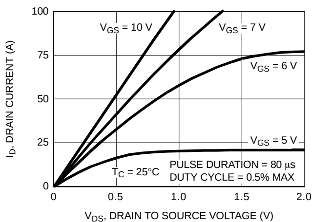
Figure 8. Saturation Characteristics
