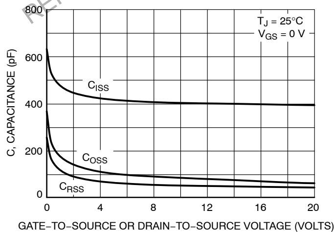
Figure 22. Capacitance Variation
