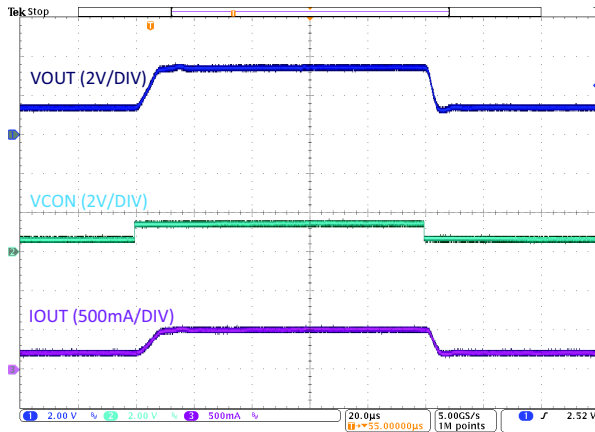
Figure 15. V_{CON} Transient (PFM to PWM), V_{OUT} = 1.4\text{ V} to 3.4\text{ V} , R_{LOAD} = 6.8\text{ }\Omega , V_{IN} = 3.8\text{ V} , 100 ns Edge
