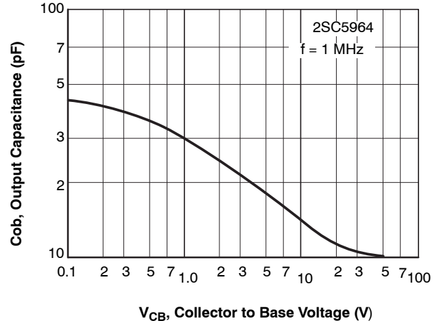
Figure 11. C_{ob} - V_{CB}
