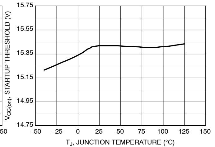
Figure 24. Startup Threshold vs. Junction Temperature
