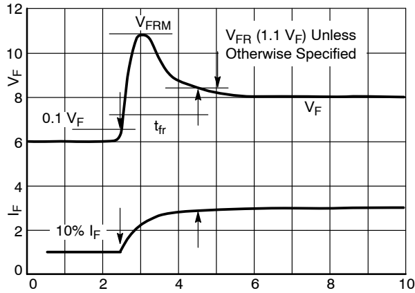
Figure 26. t fr Measurement
