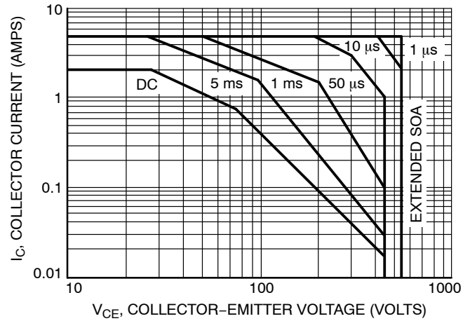
Figure 27. Forward Bias Safe Operating Area
